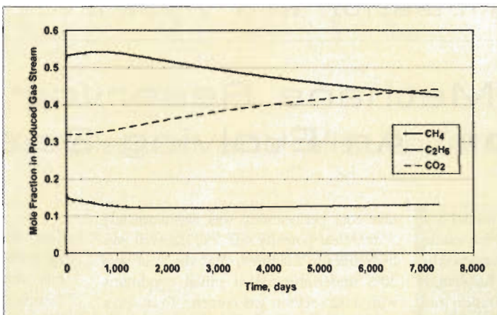
Fig. 2—Produced-gas composition predicted by a compositional CBM model.
