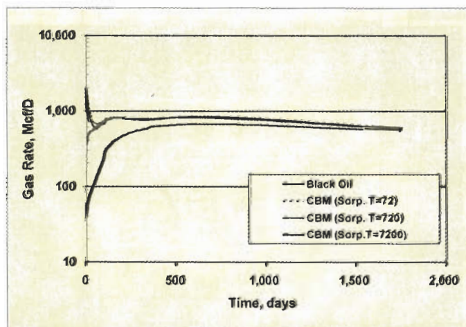
Fig. 1—Comparison of modified black-oil model and a CBM simulator.
